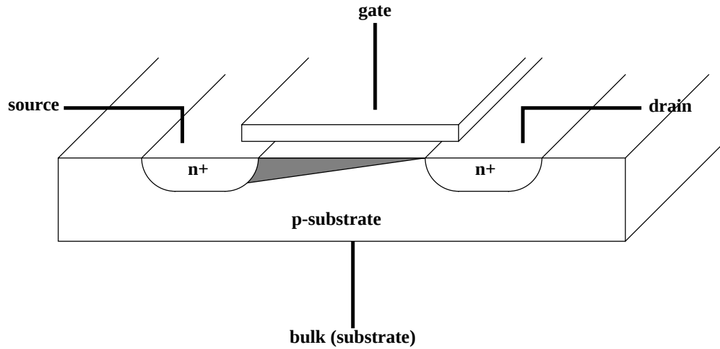
FIGURE 3. N-channel MOSFET (shown at boundary between triode and saturation)
