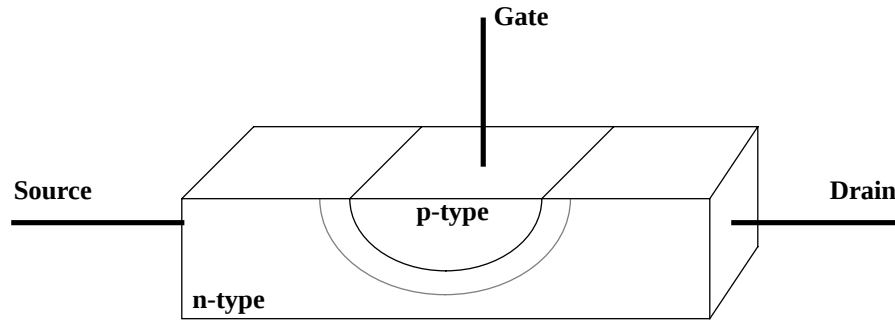
FIGURE 1. N-channel junction FET (simplified; practical devices have two gate diffusions)
