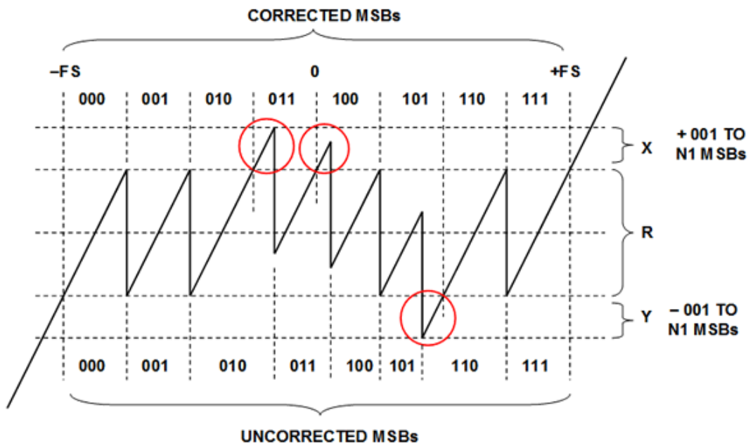
Figure 5: Error Correction Using Added Quantization Levels for N_1 = 3
