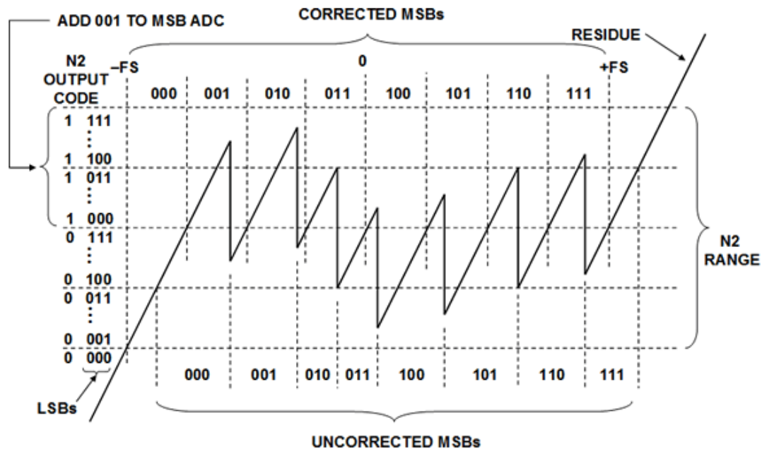
Figure 8: Residue Waveform for 6-Bit Error Corrected Subranging ADC, N1 = 3, N2 = 4, Nonlinear MSB SADC
