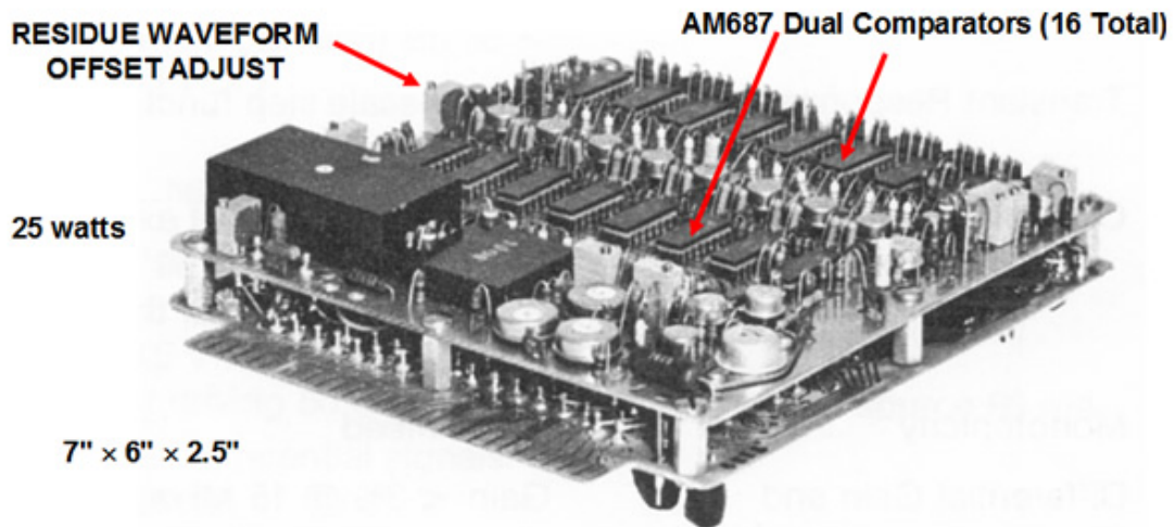
Figure 4: MOD-815, 8-Bit, 15 MSPS 4x4 Subranging ADC, 1976, Computer Labs, Inc.
