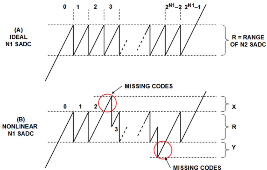
Figure 2: Residue Waveform at Input of Second-Stage SADC
