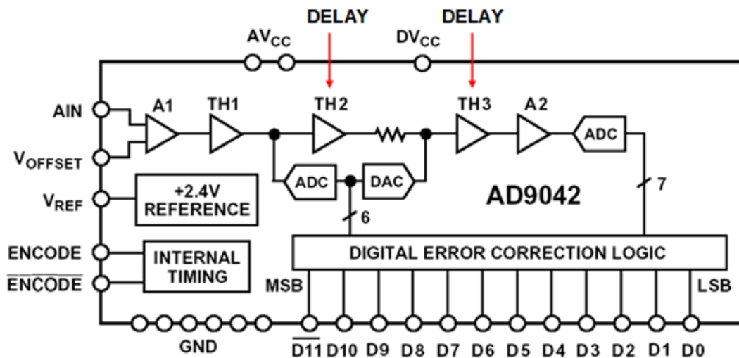
Figure 13: AD9042 12-Bit 41-MSPS ADC, 1995
