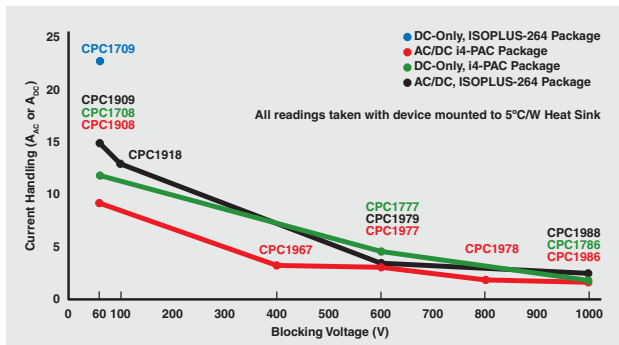
Figure 1. Clare Solid-State Relays
