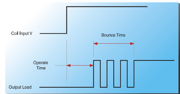
Figure 4. EMR Contact Bounce
